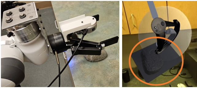
Fig. 2: A rock being scanned (left) and reconstructed as an AR mesh displayed in the headset (right). The operator can also “feel” the virtual object as the controller moves across it, as we map the reconstructed texture to vibrotactile and audio feedback.
